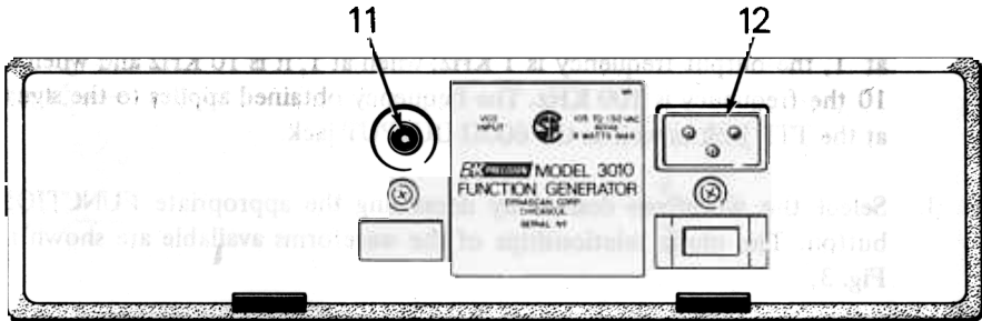
Fig. 2. Rear panel.
